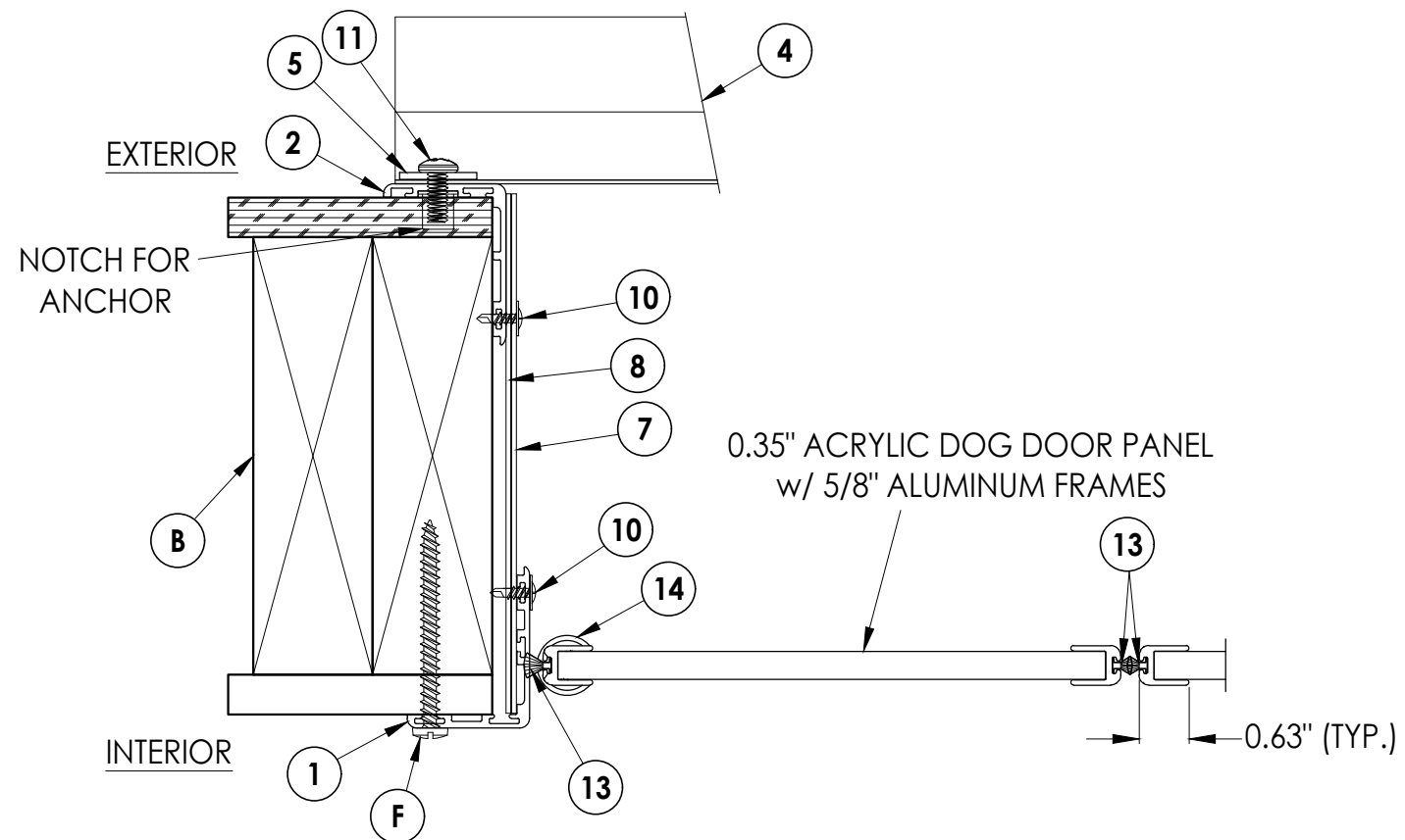
2 3 HORIZONTAL CROSS SECTION
